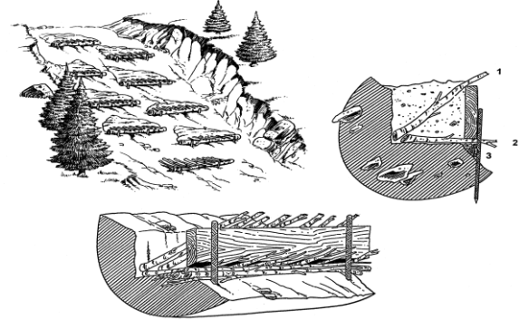
Figure 7. Modified brush layers can be built with either a log or a board for support. They should be staggered across a slope so that material rolling down the slope doesn't have a chance to get going before it is caught. The detail shows a modified brush layer prior to backfilling, while the section shows the normal backfill which creates a bit of a bench.
