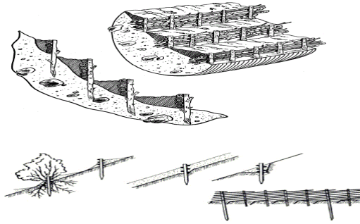
Figure 6. Wattle fences are short retaining walls constructed of living cuttings. They are used to provide slopes, which will support plant growth where over steepened slopes are preventing plant establishment. The section shows the effects of steeper slopes on wattle fence spacing.
